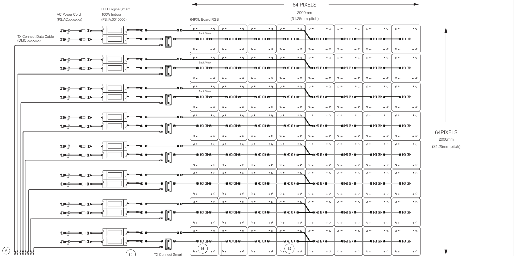
64 x 64PXL Board RGB for 2m x 2m (4 sqm)
